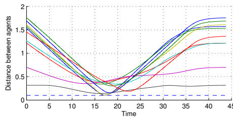
Fig. 6: Distances between agents (solid lines) and minimum safety clearance (dashed line)
