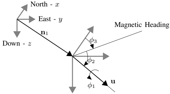
Fig. 1: Earth-Fixed Coordinates
