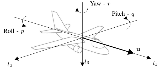
Fig. 2: Body-Fixed Coordinates
