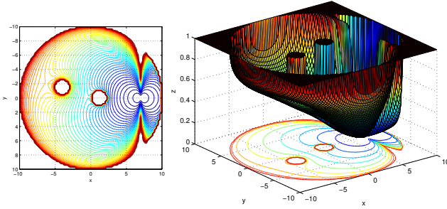
Fig. 3: 2-D Dipolar Navigation Function
